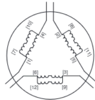
12 LEAD 230V LOW VOLTAGE MOTOR CONNECTIONS
