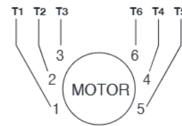
6 LEAD MOTOR CONNECTIONS
