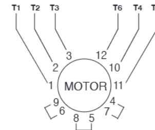
12 LEAD 460V HIGH VOLTAGE MOTOR CONNECTIONS
