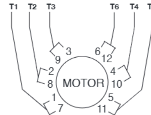
12 LEAD 230V LOW VOLTAGE MOTOR CONNECTIONS
