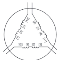
12 LEAD 460V HIGH VOLTAGE MOTOR CONNECTIONS
