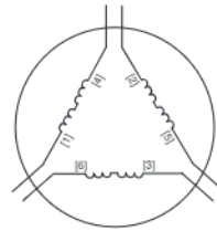
6 LEAD MOTOR CONNECTIONS
